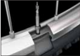
Perçage correct.
